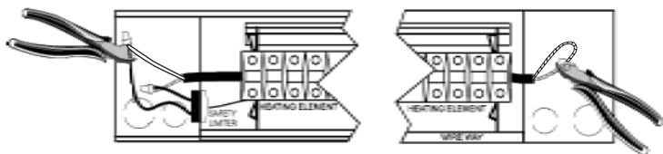
Cut one wire to Apply Power to LEFT SIDE
